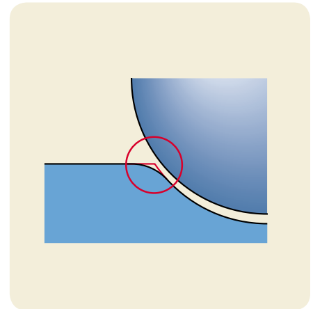
Raceway-shoulder transition
