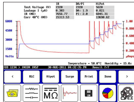
DC test results
