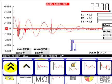
Partial Discharge (PD) test results
