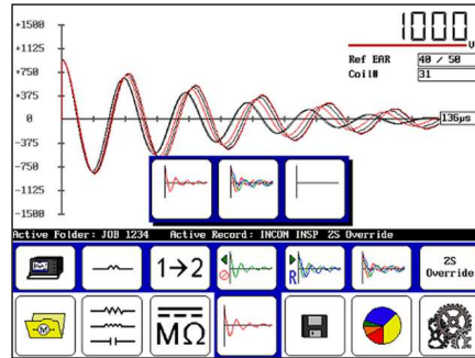
Surge test on multiple coils
