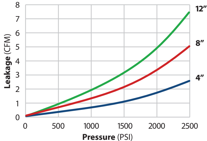
[K•DGS] Leakage rates (350 fps)
