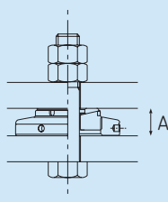
Surface treated SKF Vibracon low profile
