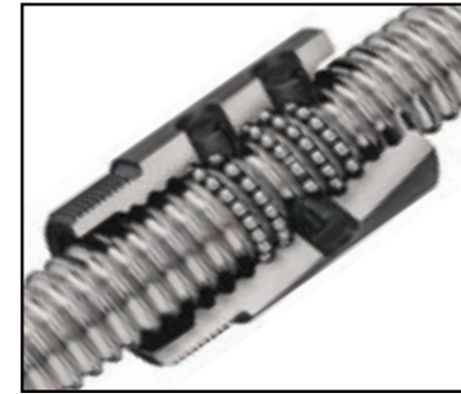
Rolled thread ball screw internal recirculation nut with threaded end.
