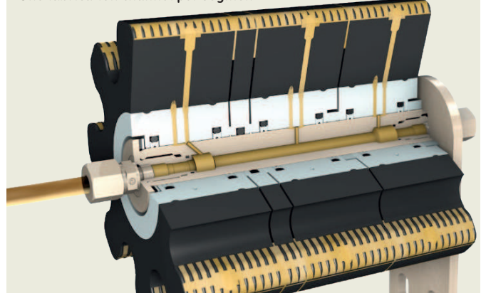
One lubrication channel per segment
