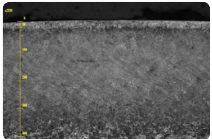
Fig. 2 Micro crack caused by fatigue 130 microns below the surface.
