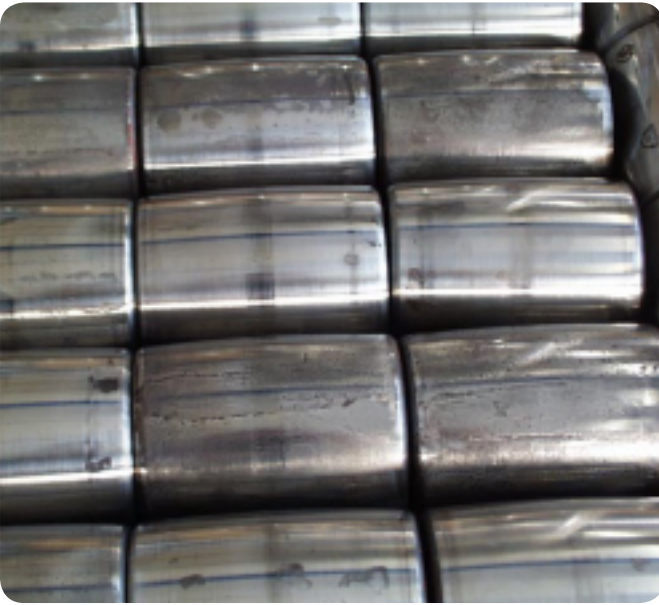
Fig. 7 The rollers of the bearing shown in figure 6
