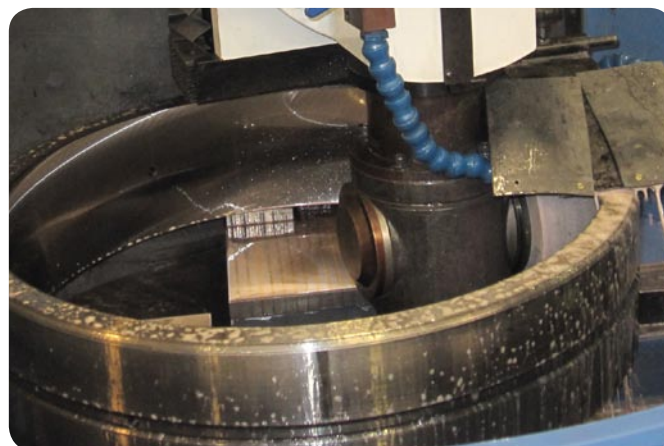
Fig. 10 Level 4 grinding of a spherical roller bearing outer ring
