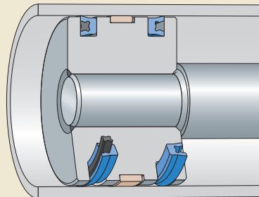
STD profiles used as piston seals (in a double-acting arrangement)
