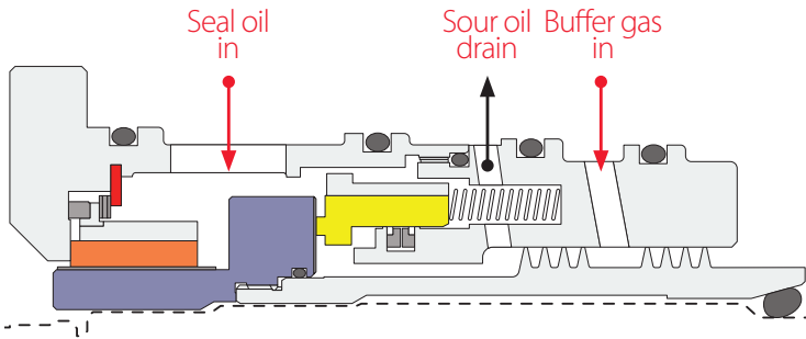
Typical arrangement for screw compressors
