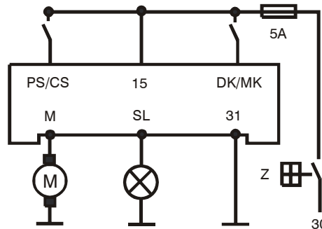
Fig. 3. Terminal connection diagram
