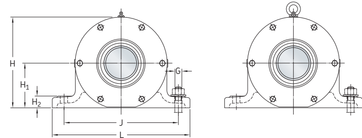
Size 320 and above (with M10 eye bolt)
