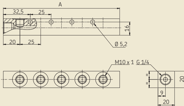
Manifold
