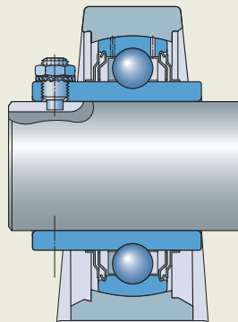
Hexagonal socket grub screw with a dog point secured by a nut and spring washer
