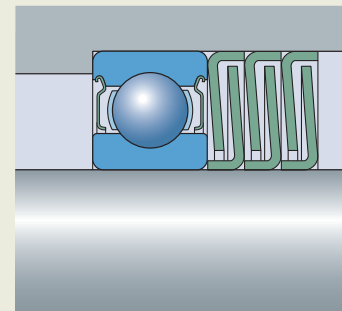
Sealing solution using SKF sealing washers
