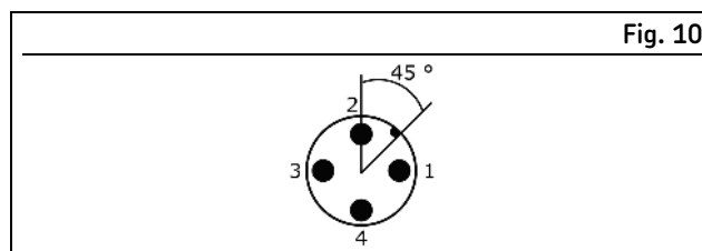
Pin assignment of M12 connector
