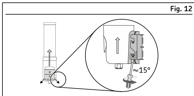
Removing the TLMR from its bracket
